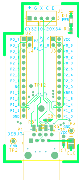
PDCR-9297 REV *A PRIMARY SIDE
